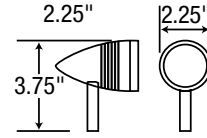
TYPE MB - MR16 Die cast 35 W max.
