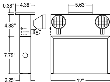
TYPE SM - PAR18 Thermoplastic 12 W max.
