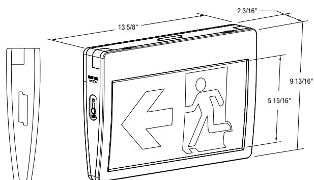
Tapered mount
