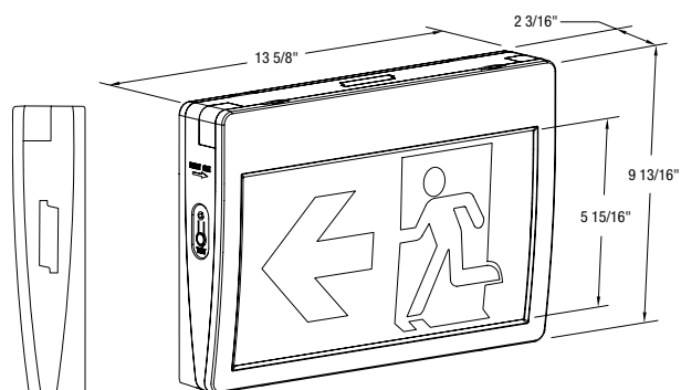
Flush mount
